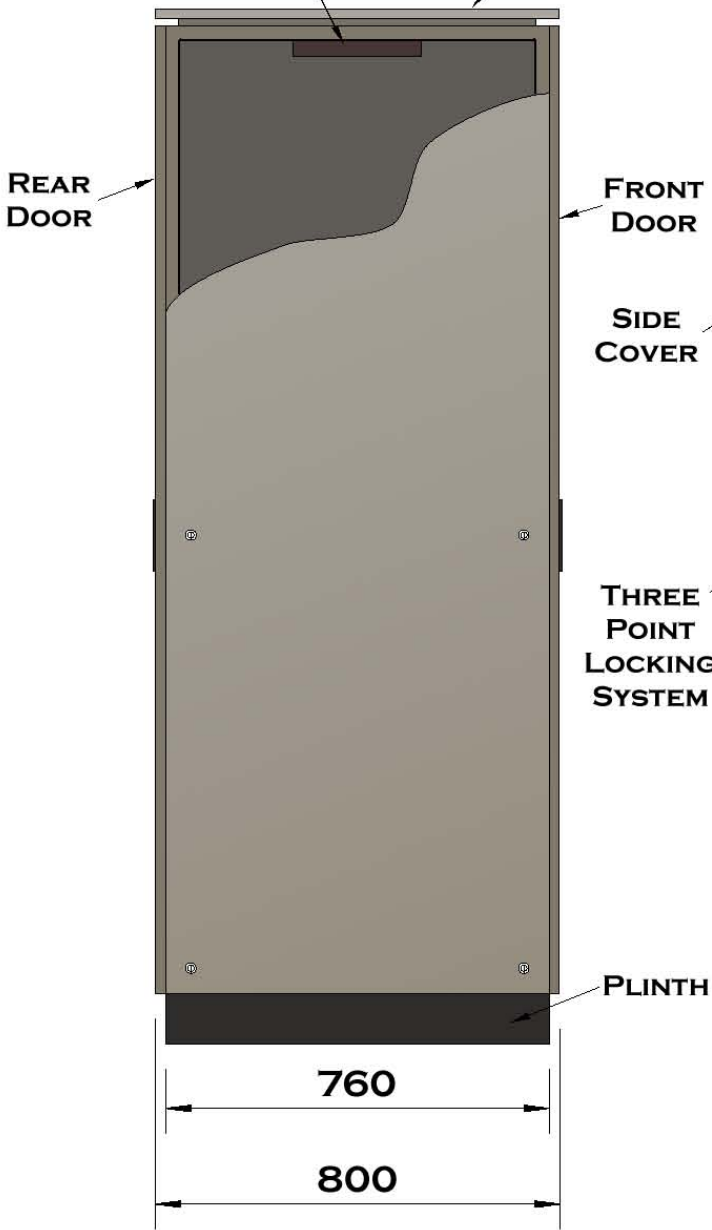
SIDE VIEW
