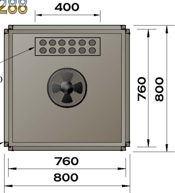
TOP SECTIONAL VIEW
